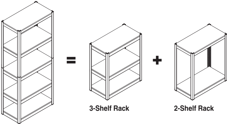
5-Shelf Rack
